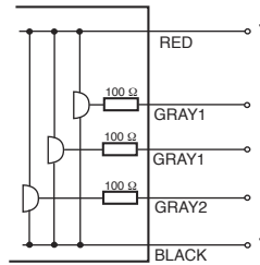
Triple 5V TTL active-high output
