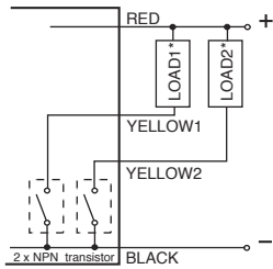
Double Open Collector (OC) output
