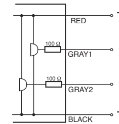
Double 5V TTL active-high output
